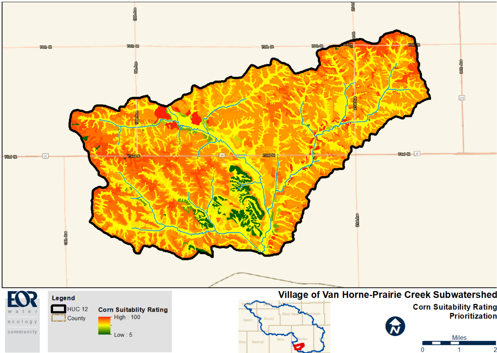
Figure 10: Corn Suitability Rating 2 for Village of Van Horne – Prairie Creek Subwatershed.
