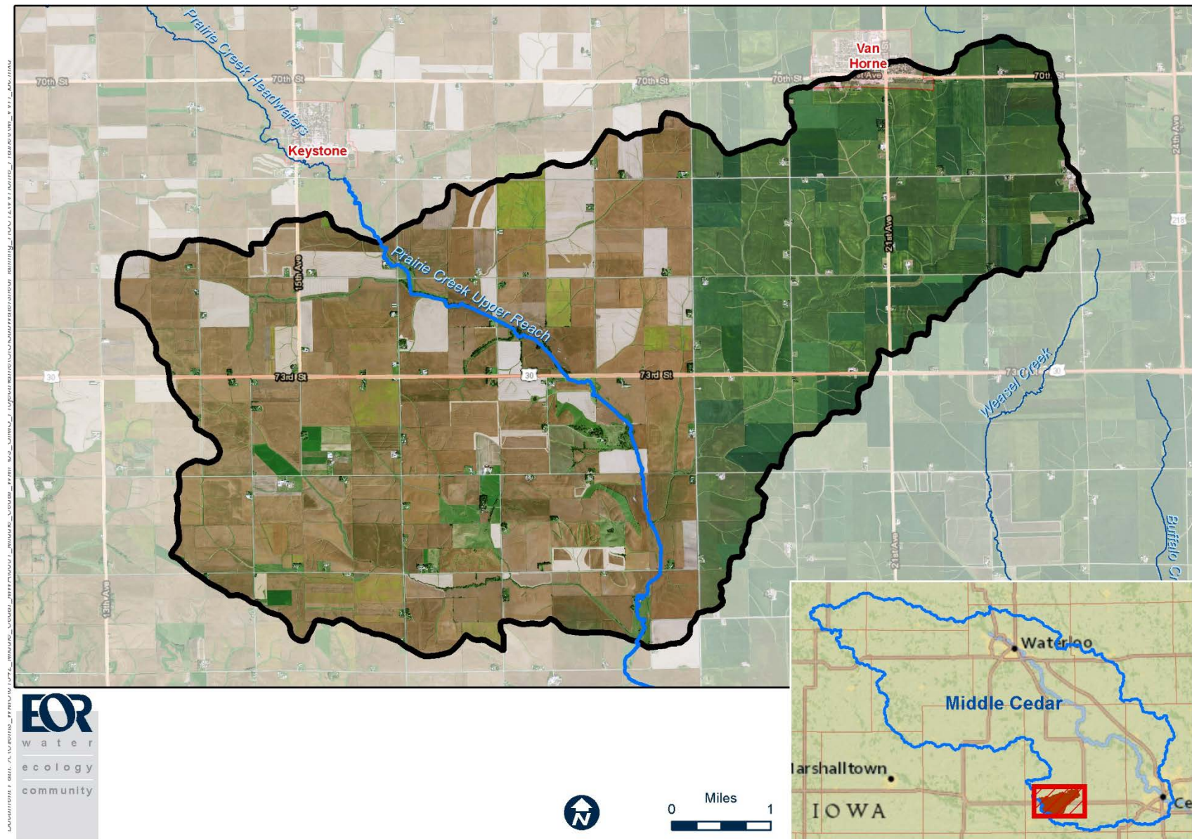
Figure 1. Village of Van Horne – Prairie Creek Subwatershed.
