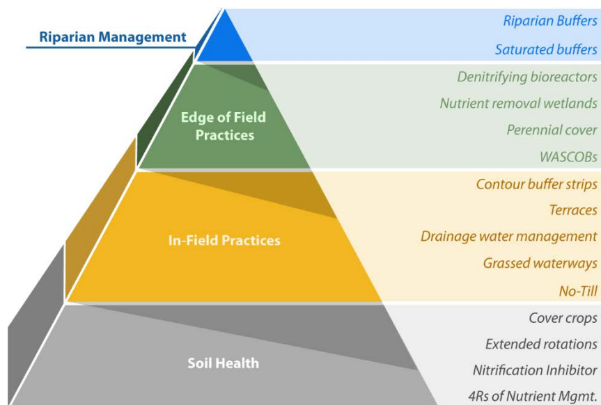
Figure 7. Conservation Pyramid (adapted from Tomer et al. 2013).
