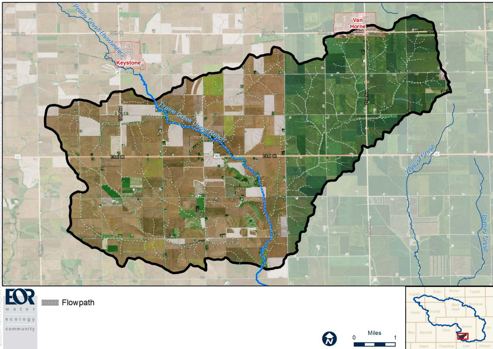
Figure 3. Water Resources of the Village of Van Horne – Prairie Creek Subwatershed.
