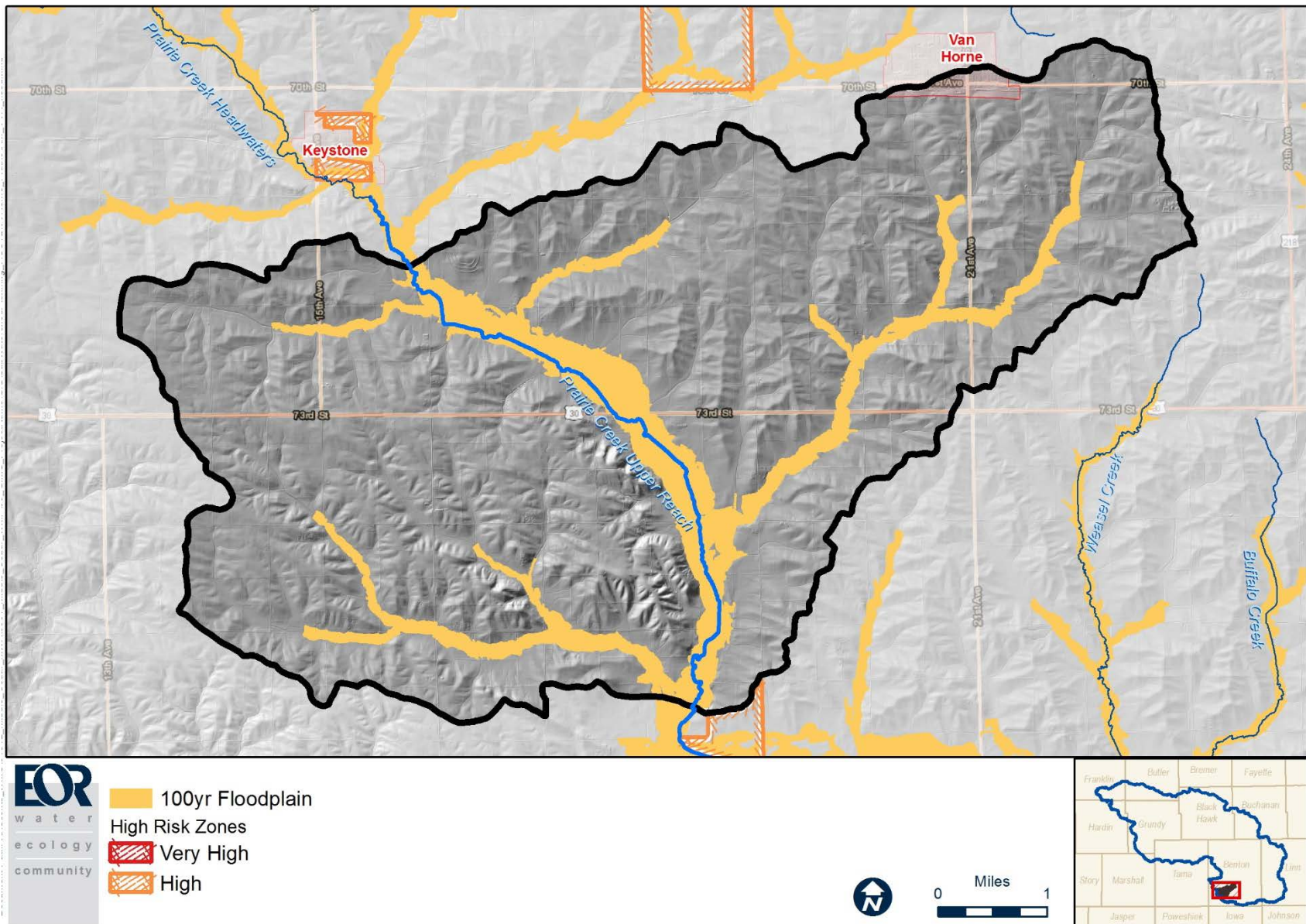
Figure 4. Flooding within the Village of Van Horne – Prairie Creek Subwatershed.
