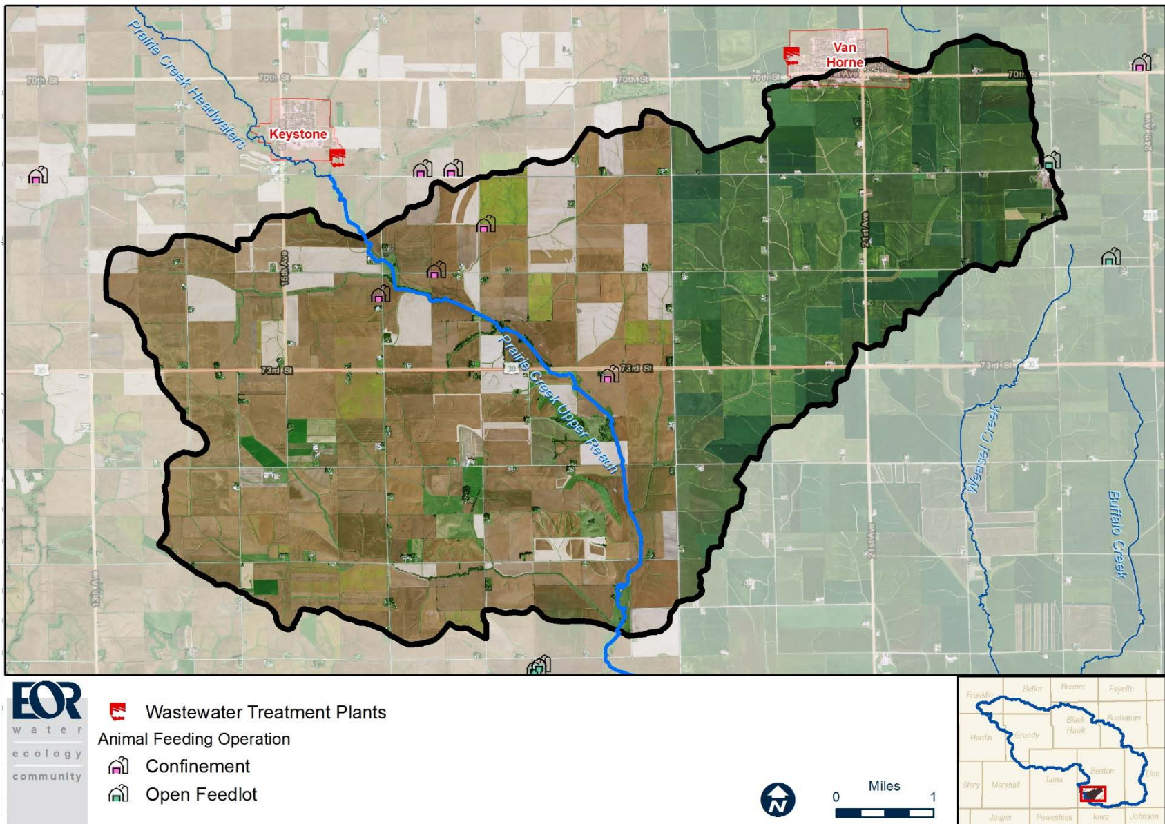
Figure 5. Wastewater Treatment Plants, Unsewered Communities and Animal Feeding Operations in the Village of Van Horne – Prairie Creek Subwatershed.
