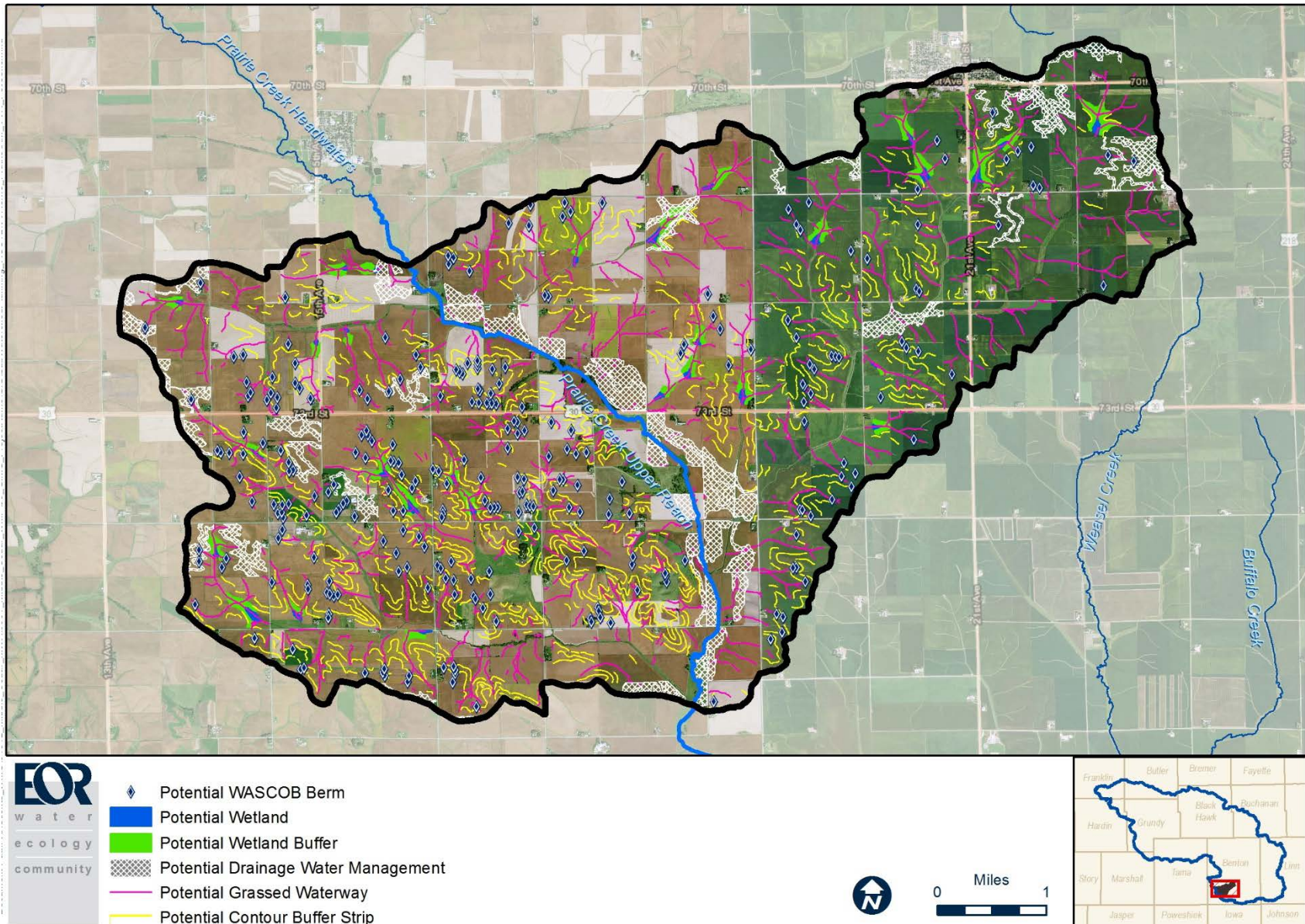
Figure 8. Potential Conservation Practices in the Village of Van Horne – Prairie Creek Subwatershed
