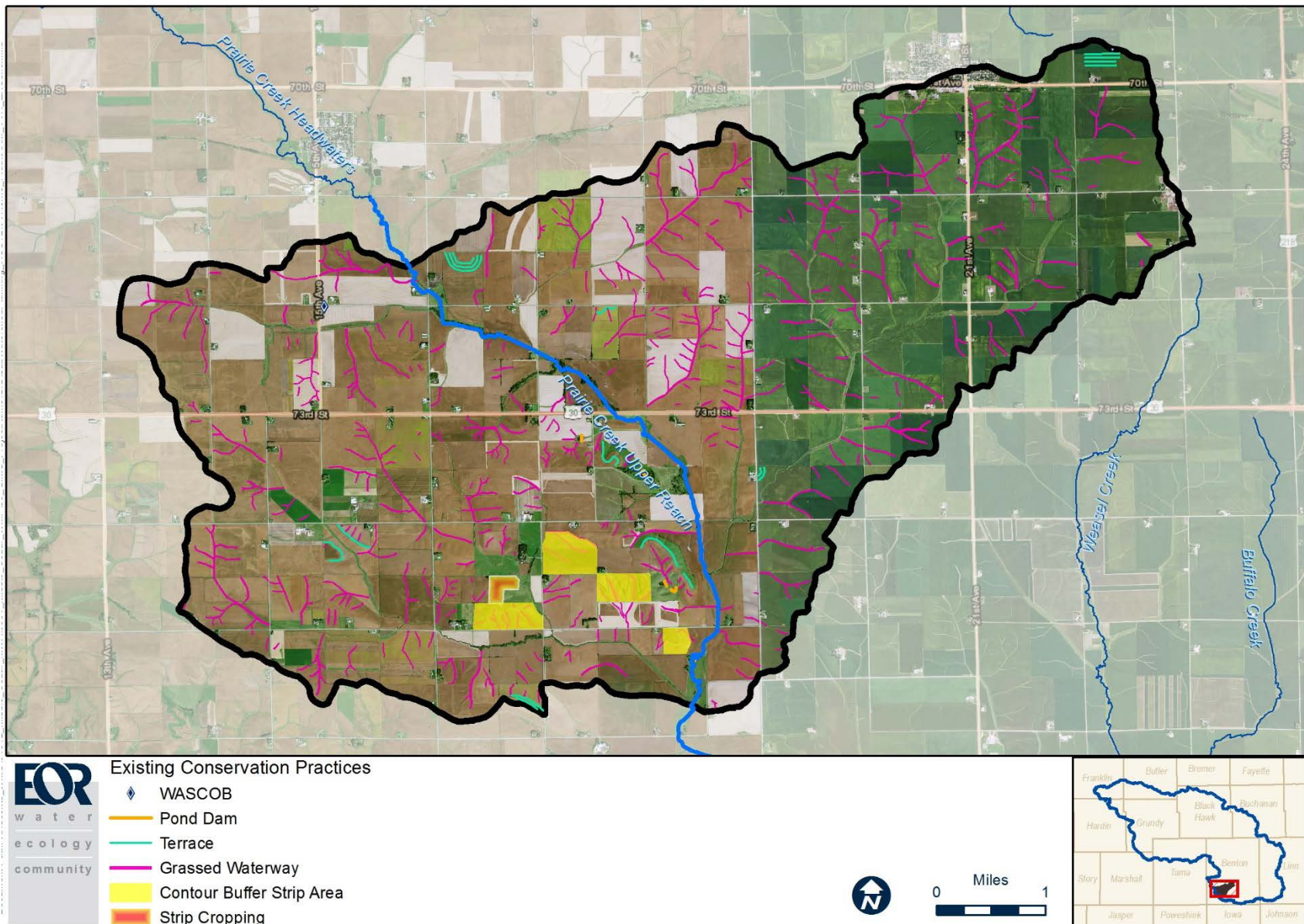
Figure 6. Existing Conservation Practices in the Village of Van Horne – Prairie Creek Subwatershed.
