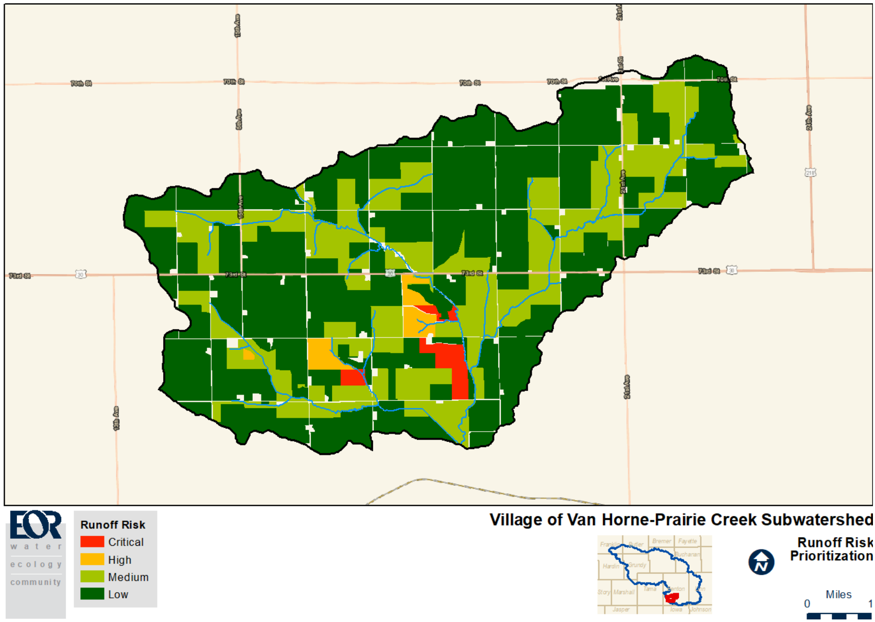
Figure 9: Runoff Risk for Village of Van Horne – Prairie Creek Subwatershed.
